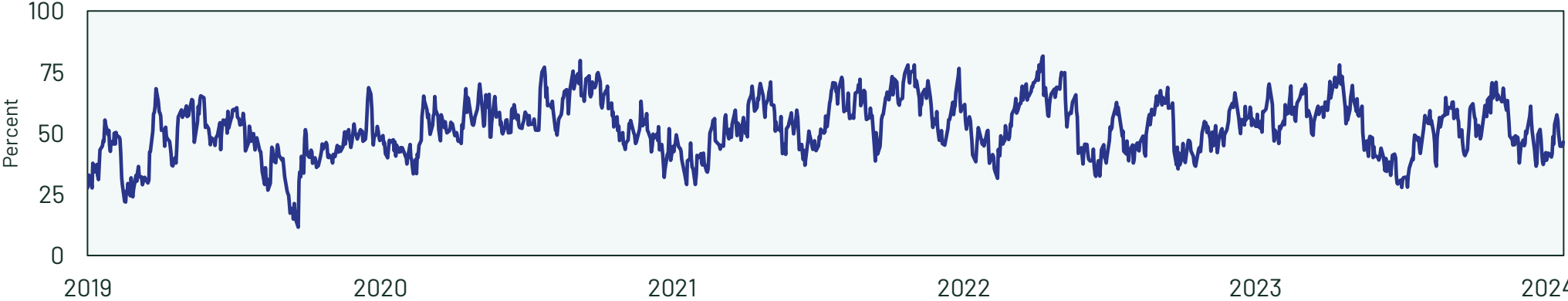
Overbought/Oversold
